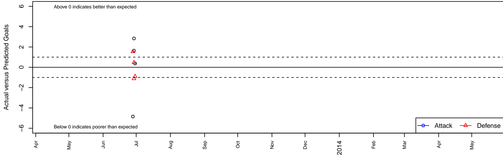
Oswego Xeneize B02 Dots are actual minus expected GF (blue circles) and GA (red triangles). Blue line is smoothed change in attack strength. Red is smoothed change in defense strength.
